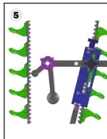
Ideal equipment: the quick tensioning device (3) for easy release, changing and cleaning of the cup belts.
