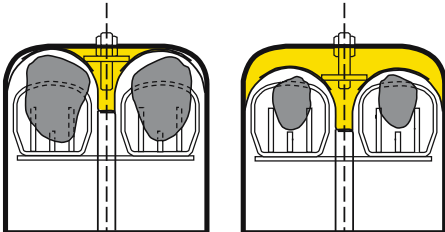
If it doesn't fit, we make it fit: the adjustable drop trunks. Narrow for small seed and wide for large seed.
